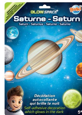
2013DF4 (6) Glow-in-the-dark Saturn | Saturne
