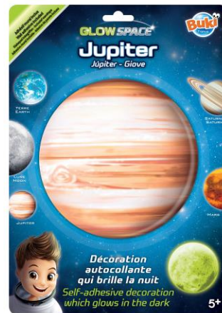
2013DF6 (6) Glow-in-the-dark Jupiter
